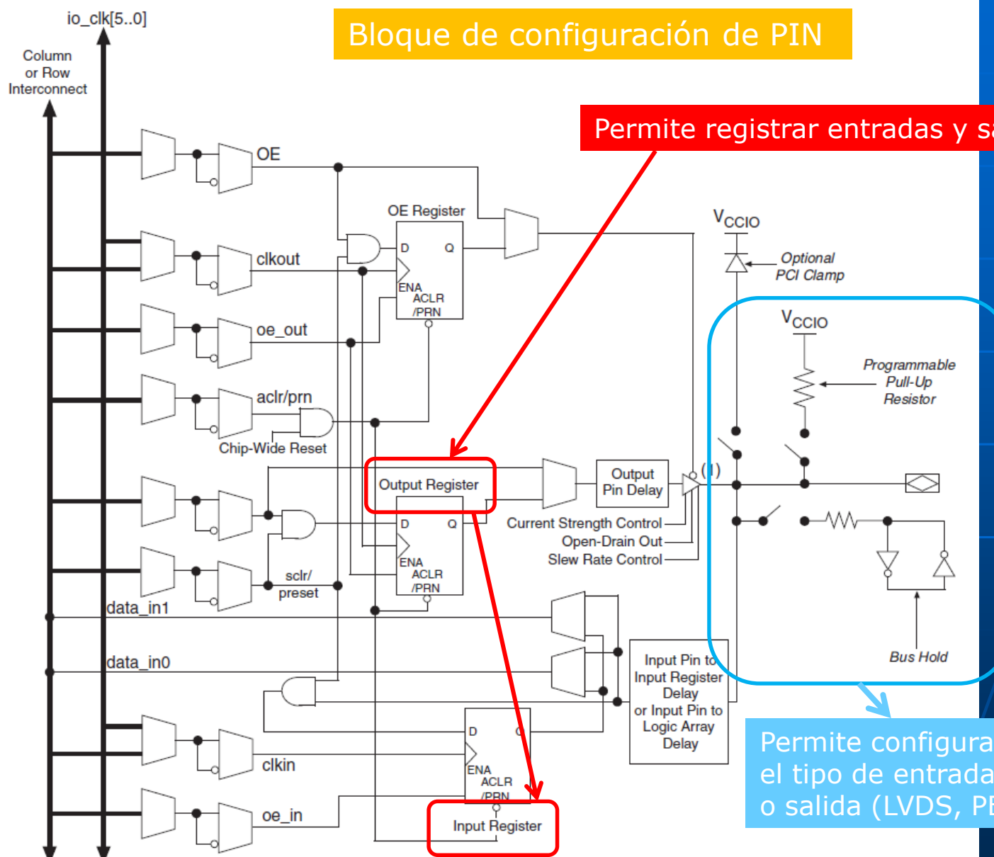
Figure 6-1. Cyclone IV IOEs in a Bidirectional I/O Configuration for SDR Mode
